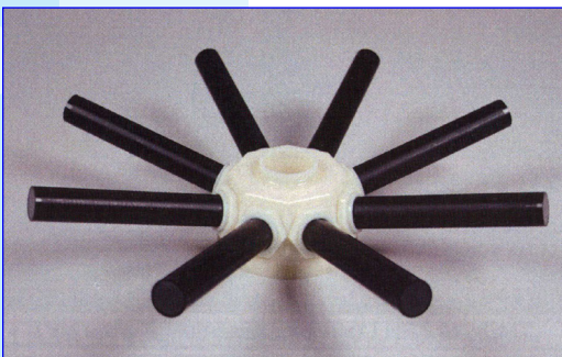
P/N: 703008 Hub and Lateral Plastic Distributor 1-1/2" diameter SCH40 PVC with 0.012" slots
